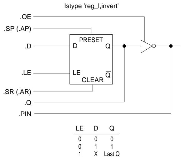
Figure 6-8 Detailed Dot Extensions for a Latch with Active Low Latch Enable
