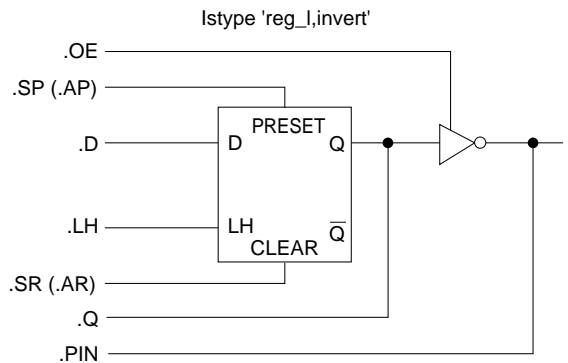
Figure 6-7 Detailed Dot Extensions for a Latch with Active High Latch Enable
