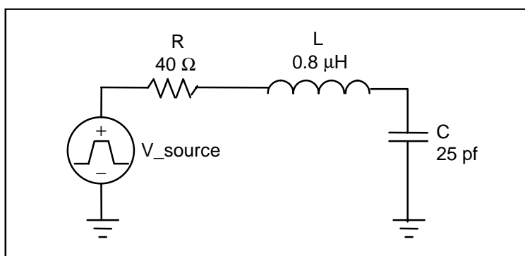
Figure D.22 – Simple RLC model of 40-conductor cable with all data lines switching
